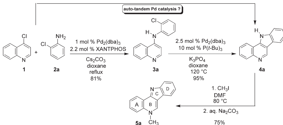
Scheme 1. Synthesis of 4a via consecutive palladium-catalyzed reactions.
