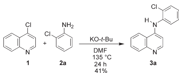
Scheme 2. Synthesis of N -(2-chlorophenyl)quinolin-4-amine ( 3a ) via nucleophilic aromatic substitution.
